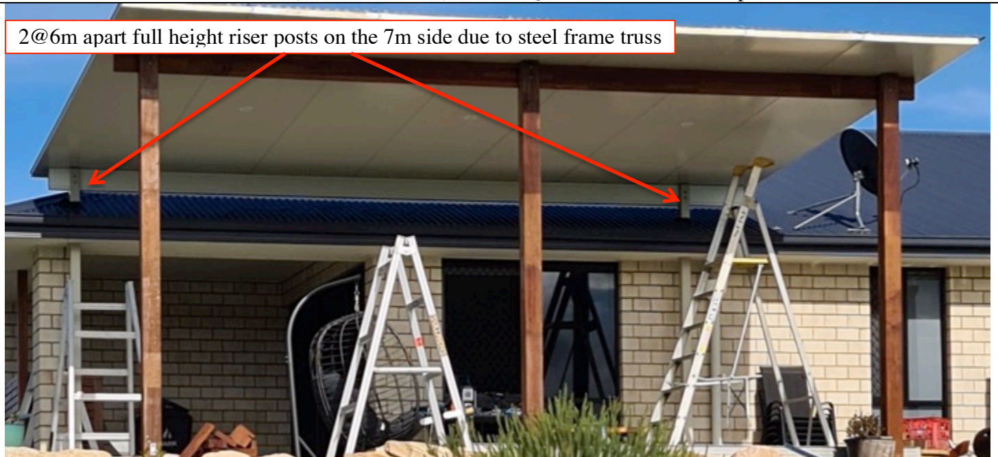
FULL HEIGHT RISER POSTS (steel truss house) HOYA QLD – Case A 3 sides open N3 50mm Insulroof®
