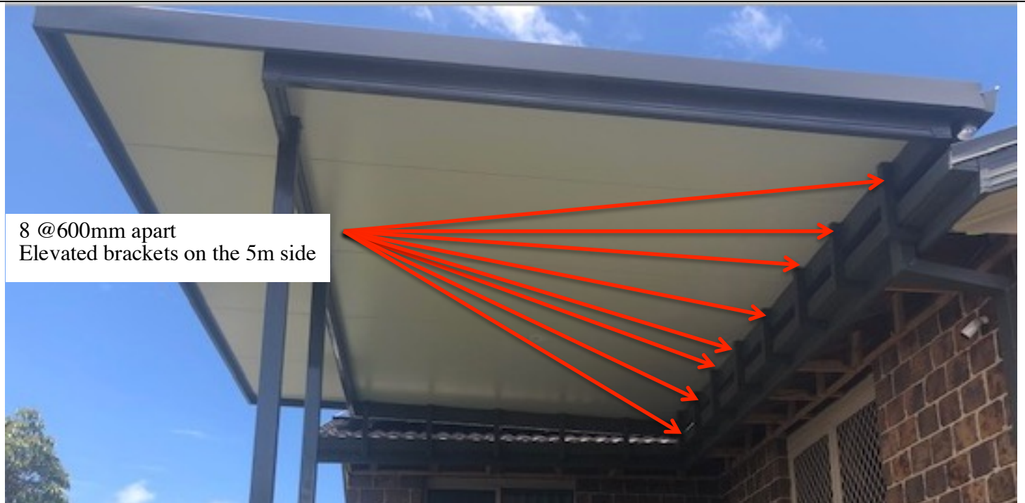
ROOFEXTENDA® – CARIINGTON NSW – 5@5000mm Case B 2side closed N3 100mm Solarspan®
